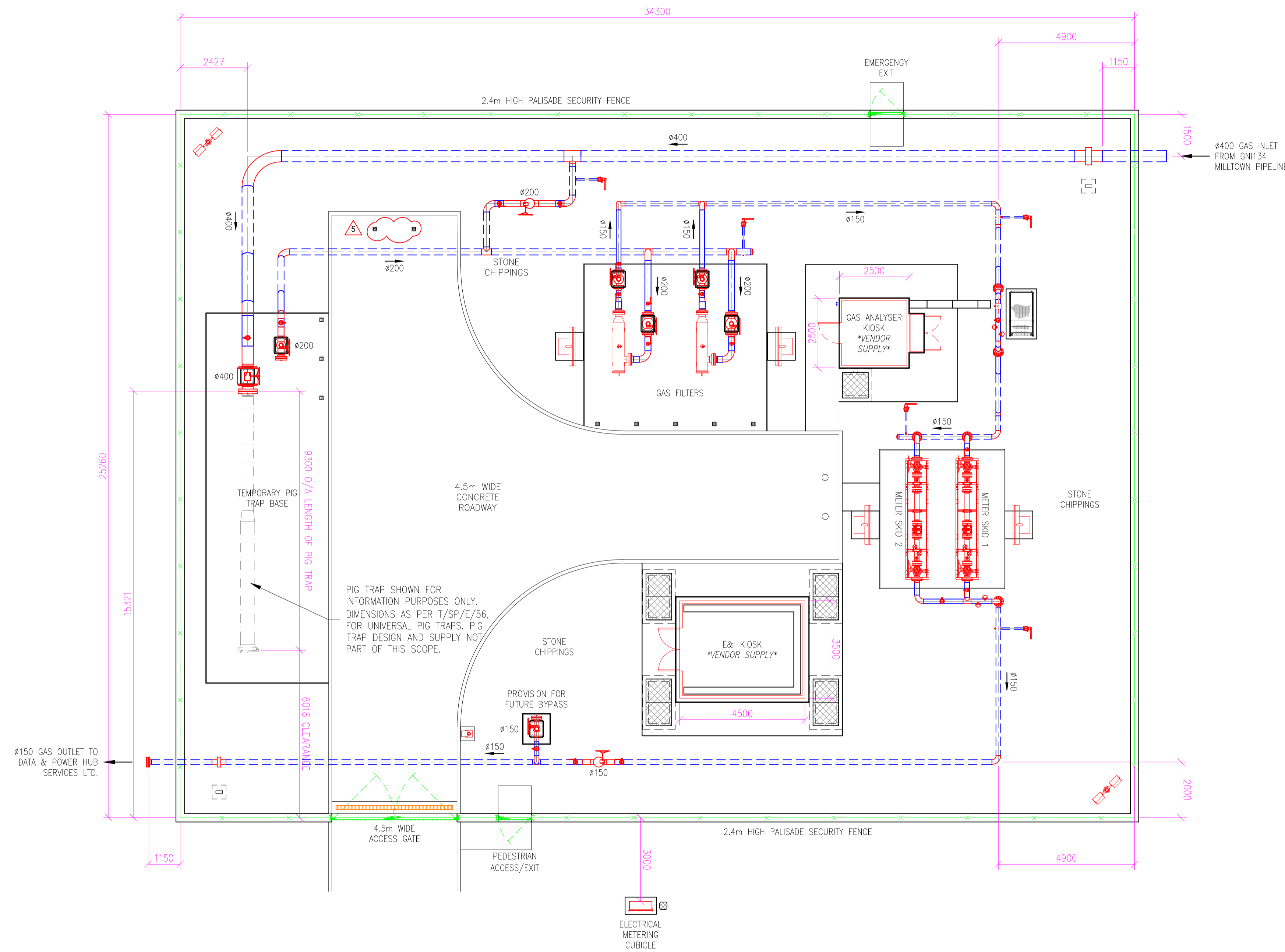
PLAN OF AGI (Scale 1:100)
