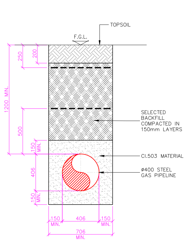
TYPICAL REINSTATEMENT DETAIL FOR Ø400 PIPELINE (GRASS VERGE EXCAVATION) (Not to Scale)
