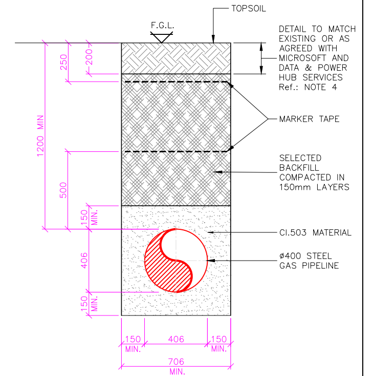
TYPICAL REINSTATEMENT DETAIL FOR 400mm PIPELINE (MICROSOFT AND DATA & POWER HUB SERVICES SITES) (Not to Scale)
