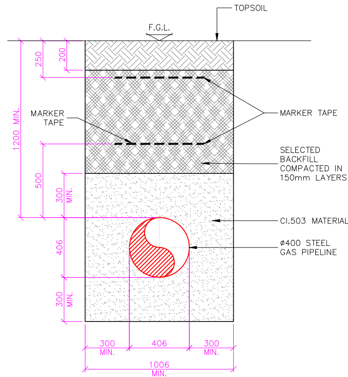
TYPICAL REINSTATEMENT DETAIL FOR Ø400 PIPELINE (ROCK EXCAVATION) (Not to Scale)
