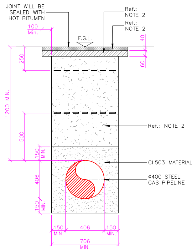
TYPICAL REINSTATEMENT DETAIL FOR Ø400 PIPELINE (IN ROAD/FOOTPATH EXCAVATION) (Not to Scale)
